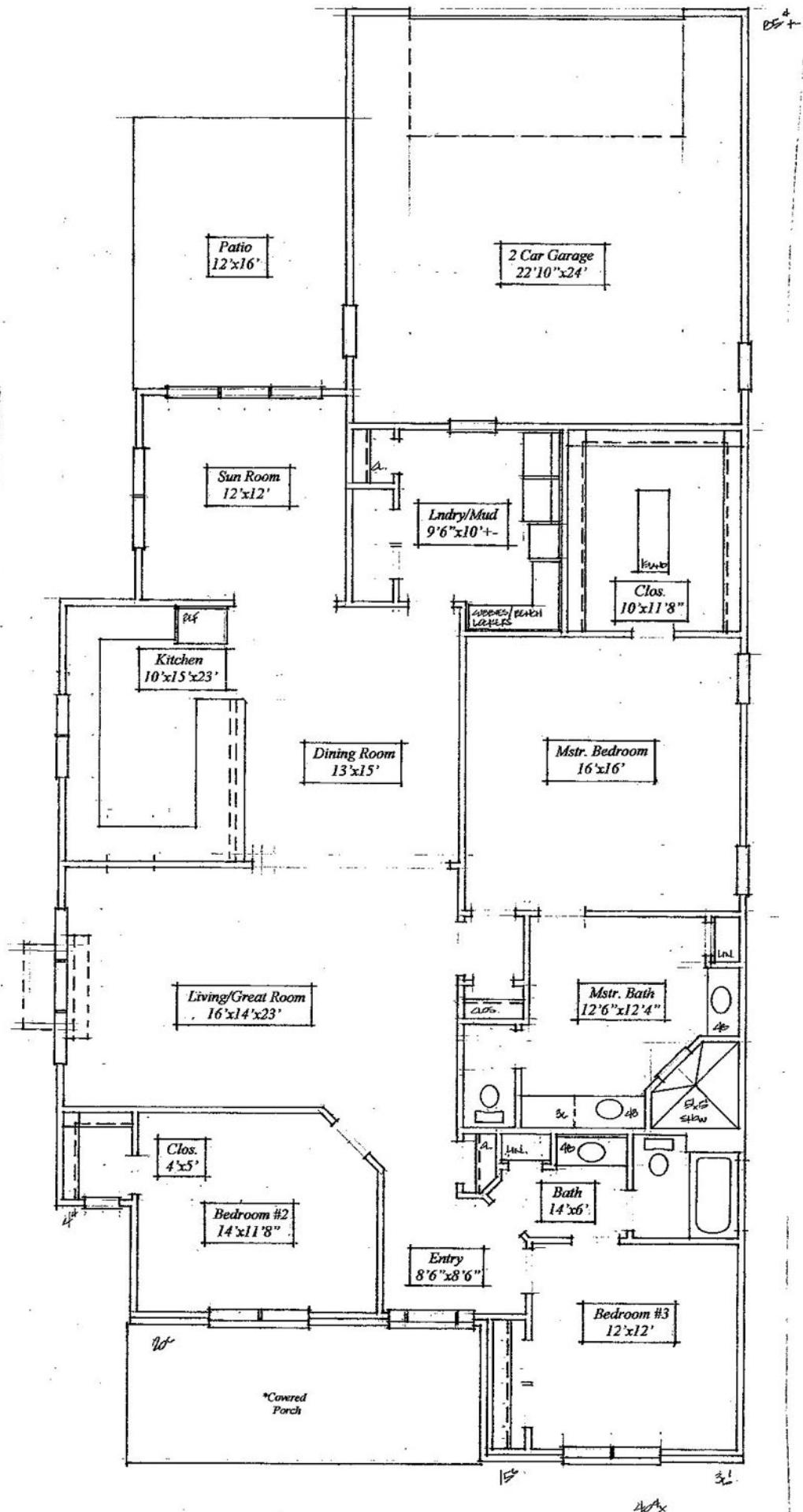
Main Level Floor Plan Preliminary
